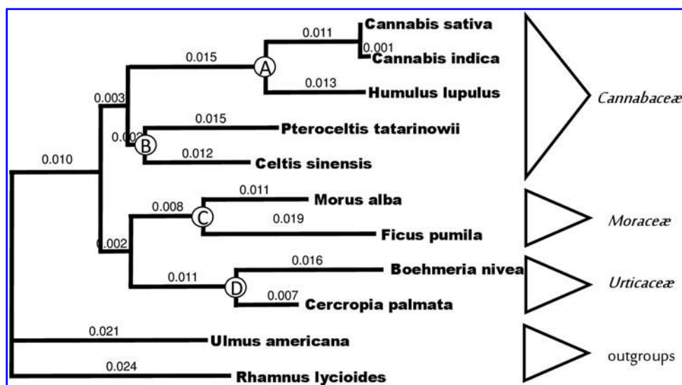
FIG. 2. Phylogenetic tree used for calculating divergence dates.
